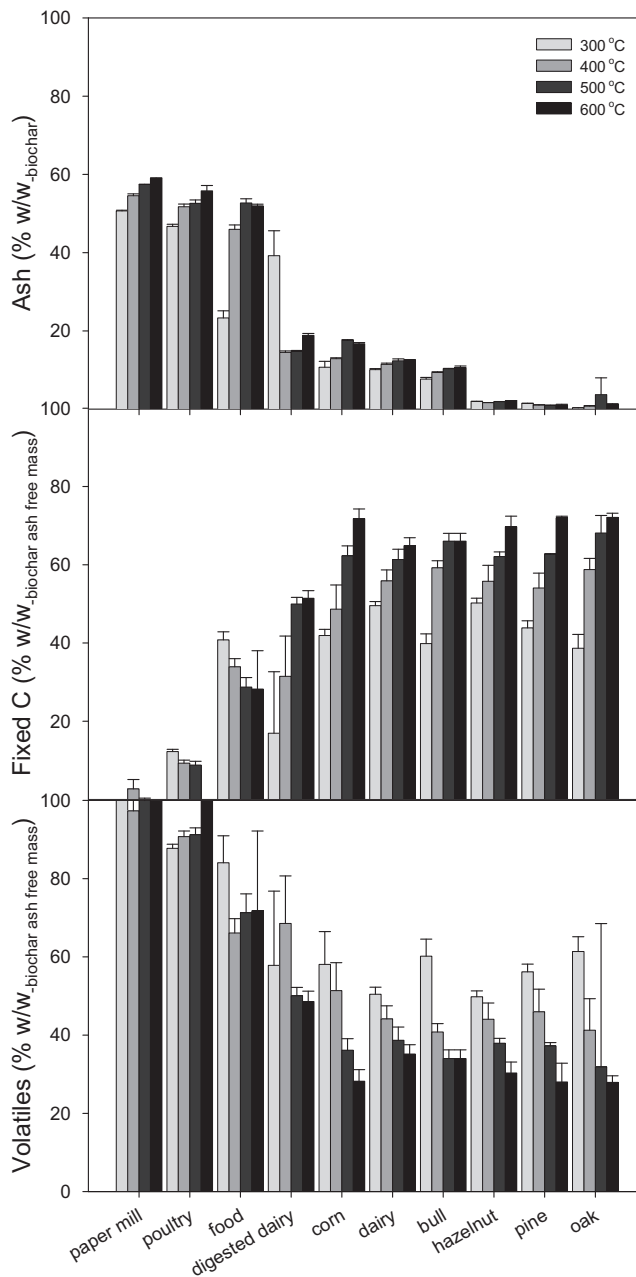
Fig. 1. Ash, volatile and fixed carbon contents (w/w) of biochars generated from different feedstocks at varying temperatures ( n = 2 ).
