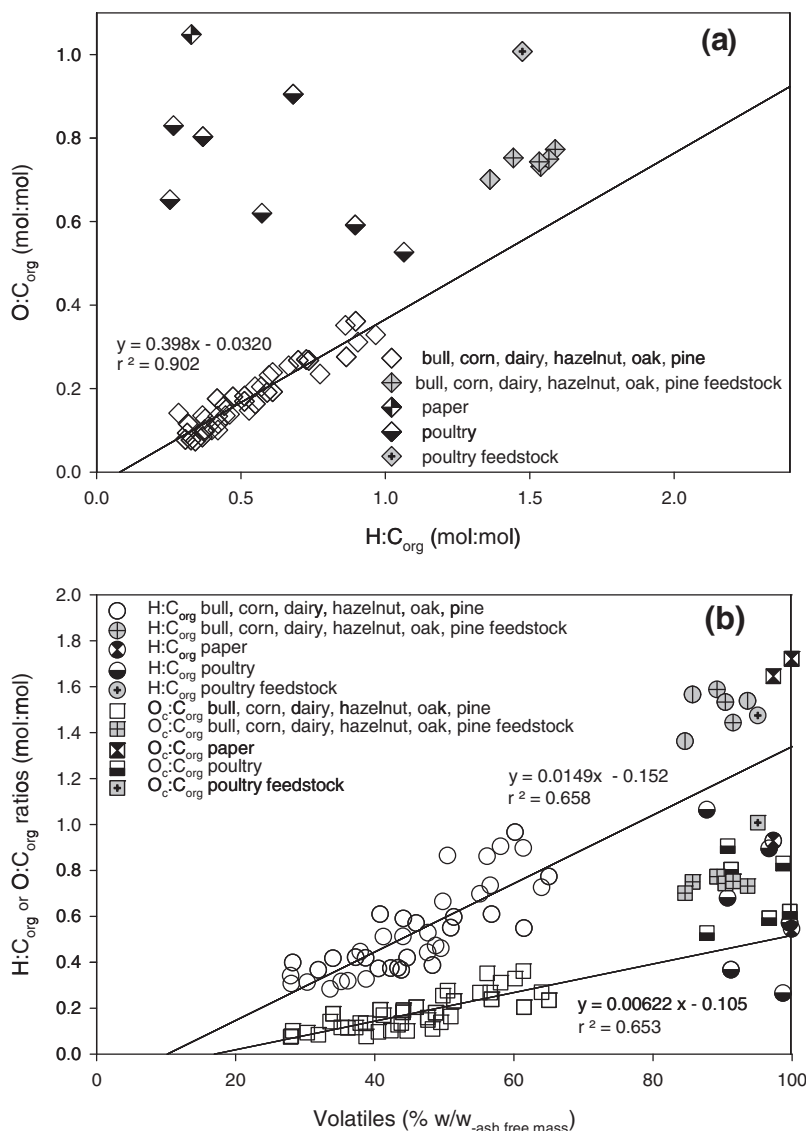
Fig. 2. Relationship between O:C org and H:C org (a) and to volatile matter (b) for different biochars and their feedstocks (n = 2).
