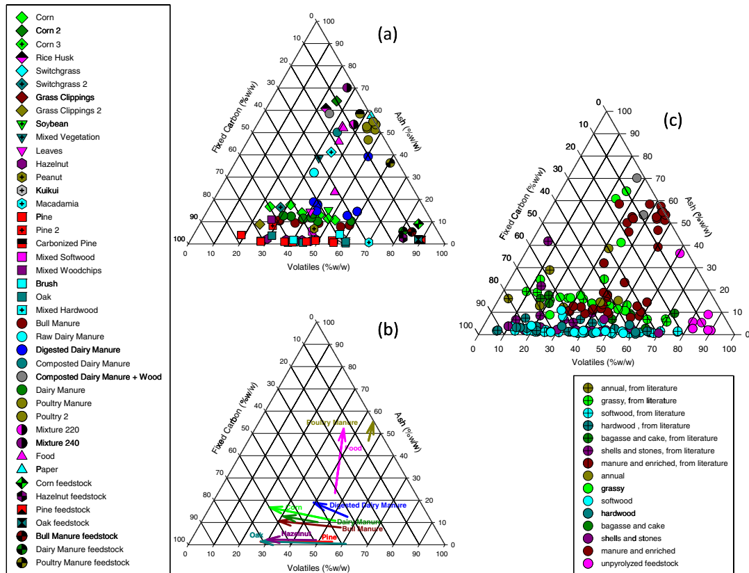
Fig. 6. Triangle plots of ash, volatile matter and fixed carbon contents (a) (sources listed in Supplementary Table S1); the effect of pyrolysis temperature (b) ( n = 2 ; arrows connect biochars of the same feedstock pyrolyzed at 300 and 600 °C); and a comparison between data from this study to literature data (c). Literature values listed in Supplementary Table S2.
