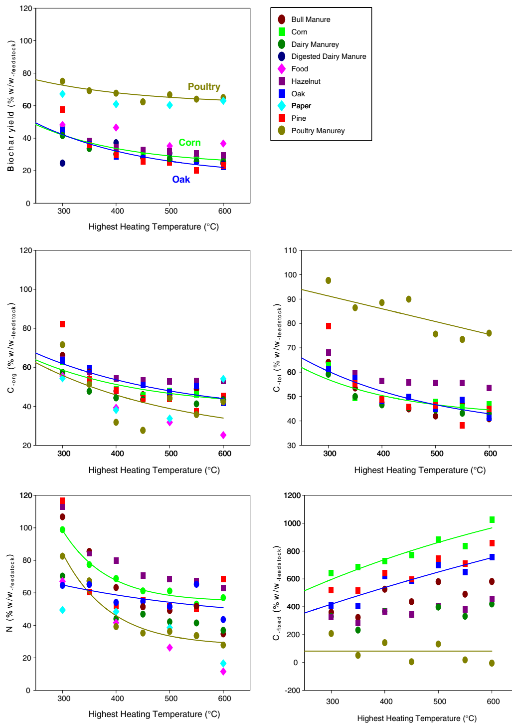
Fig. 3. Recovery of mass, total and organic C, total N and fixed carbon per unit weight of the same parameter in the feedstock with increasing pyrolysis temperature using slow pyrolysis ( n = 2 for elemental contents, n = 1 for mass; regressions with two-parameter exponential equations to improve clarity; regressions through feedstock except for N).
