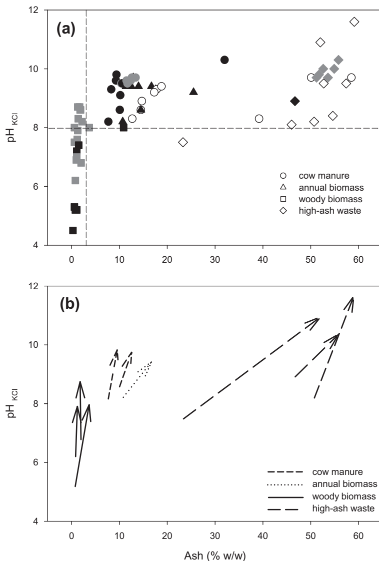
Fig. 5. Relationship between ash content and pH values (black symbols indicate CEC greater and gray symbols those lower than the median value of 265 \text{ mmol kg}^{-1} ; no CEC data available for biochars shown with open symbols) (a), and the effect of increasing pyrolysis temperature (b) ( n = 2 ; arrows connect biochars of the same feedstock pyrolyzed at 300 and 600 °C).
