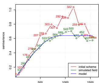
Variograms, log(Zn)
