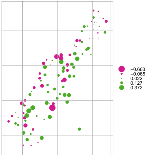
CK evaluation errors, log10(Pb), co-variable log10(OM)
