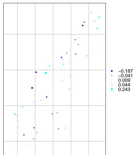
CK cross-validation errors, log10(Pb), co-variable log10(Zn)
