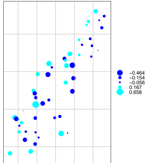
CK cross-validation errors, log10(Pb), co-variable log10(OM)
