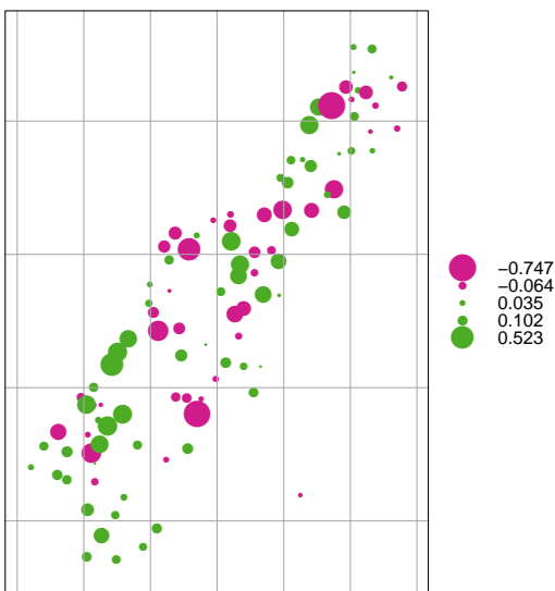
CK evaluation errors, log10(Pb), co-variable log10(Zn)
